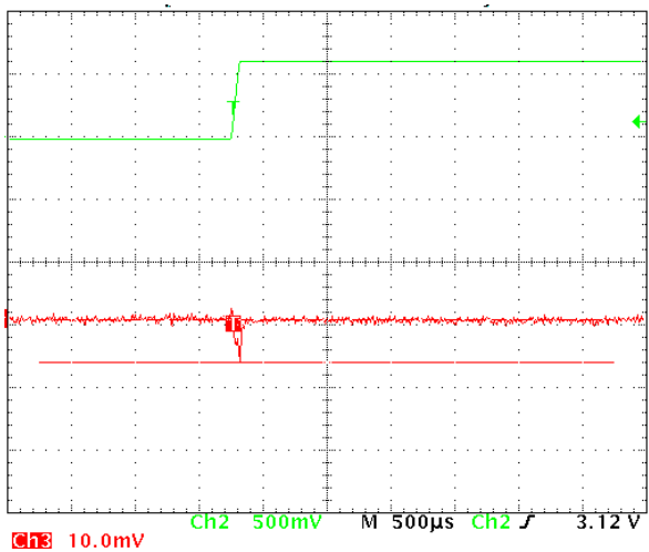
Figure 18. 3.0 V to 3.6 V Line Transient, Rise = 50 \mu\text{s} ( V_{IN} = 1.2 \text{ V} , I_{OUT} = 100 \text{ mA} , Temperature = 25^\circ\text{C} )
