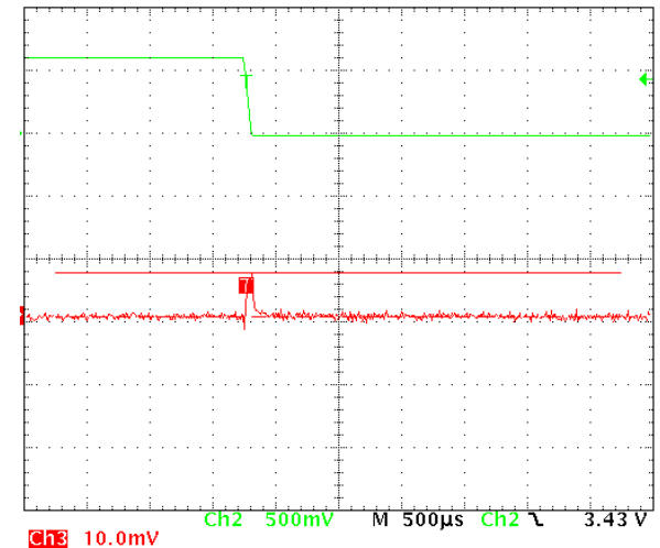
Figure 19. 3.6 V to 3.0 V Line Transient, Fall = 50 \mu\text{s} ( V_{IN} = 1.2 \text{ V} , I_{OUT} = 100 \text{ mA} , Temperature = 25^\circ\text{C} )
