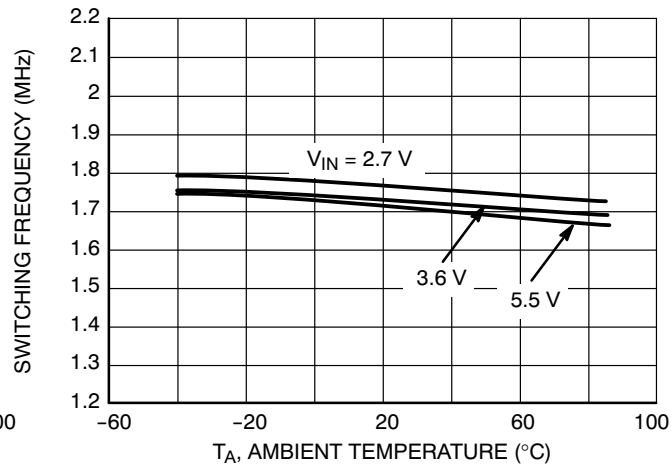
Figure 13. Switching Frequency vs. Ambient Temperature ( V_{out} = 1.2\text{ V} , I_{out} = 200\text{ mA} )
