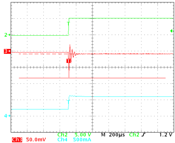
Figure 17. 200 mA to 600 mA Load Transient in 1 \mu\text{s} ( V_{IN} = 3.6 \text{ V} , V_{OUT} = 1.2 \text{ V} , Temperature = 25^\circ\text{C} )
