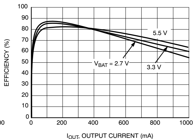
Figure 11. Efficiency vs. Output Current ( V_{IN} = 1.2\text{ V} , Temperature = 25°C)
