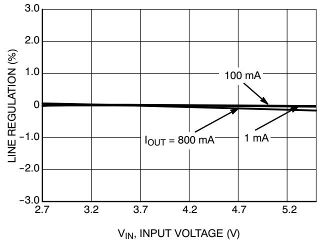
Figure 15. Line Regulation vs. Output Current ( V_{OUT} = 1.2 \text{ V} , Temperature = 25^\circ\text{C} )
