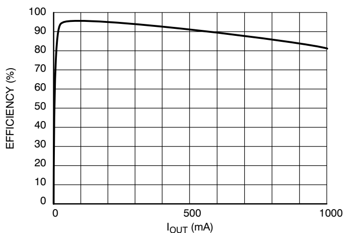
Figure 4. Efficiency vs Output Current V_{IN} = 3.6 V, V_{OUT} = 3.3 V
