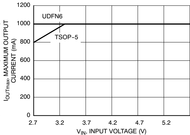
Figure 6. Maximum Output Current, T_A = 45^{\circ}\text{C}
