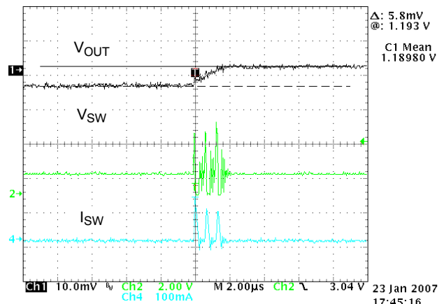
Figure 26. PFM Switching Waveforms ( V_{IN} = 3.6\text{ V} , V_{OUT} = 1.2\text{ V} , I_{OUT} = 0\text{ mA} , Temperature = 25°C)
