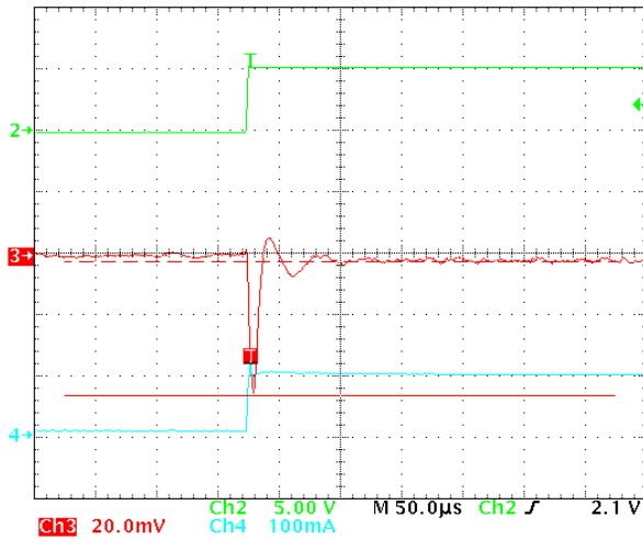
Figure 16. 10 mA to 100 mA Load Transient in 1 \mu\text{s} ( V_{IN} = 3.6 \text{ V} , V_{OUT} = 1.2 \text{ V} , Temperature = 25^\circ\text{C} )
