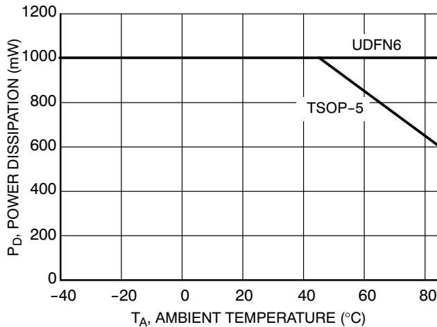
Figure 7. Power Derating
