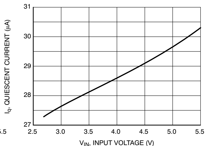
Figure 9. Quiescent Current vs. Input Voltage (Open Loop, Feedback = 1, Temperature = 25°C)
